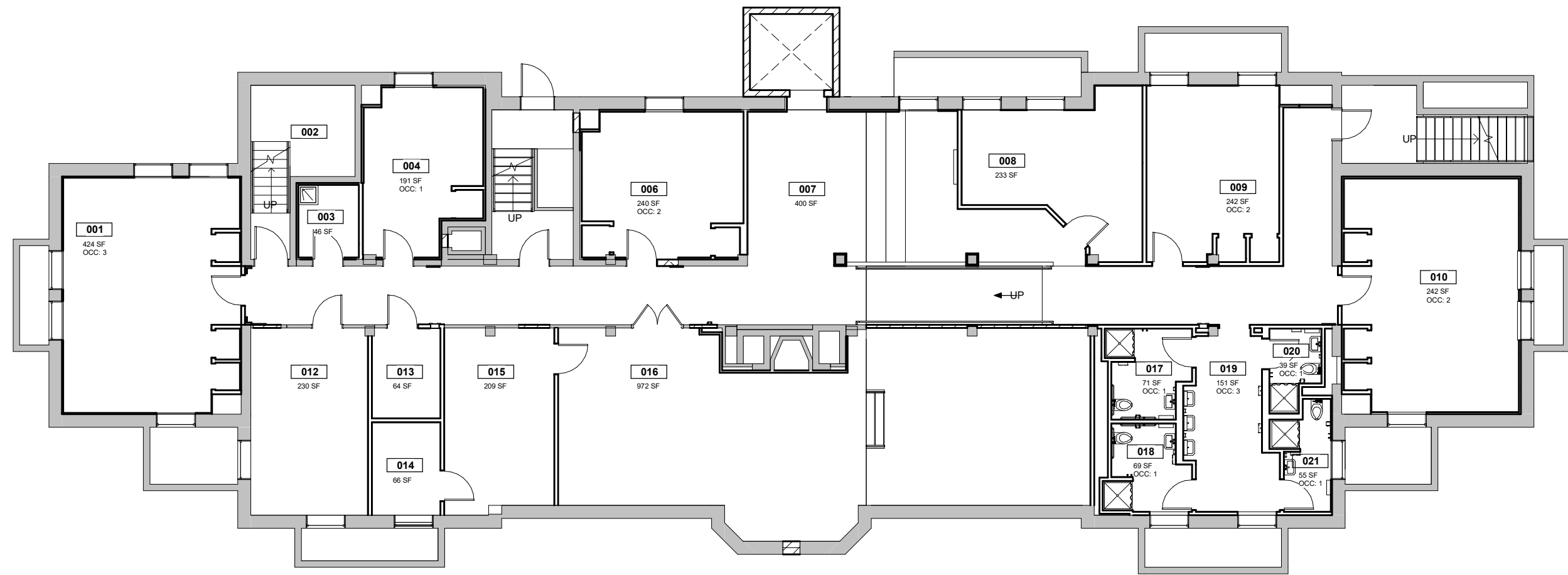
BASEMENT FLOOR PLAN
