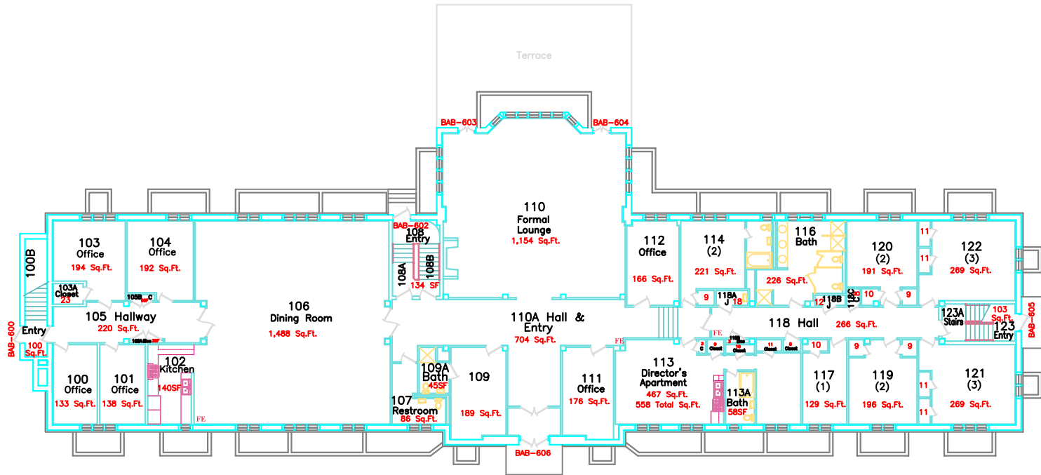
FIRST FLOOR
