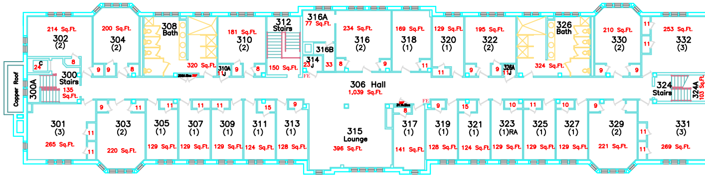
THIRD FLOOR
