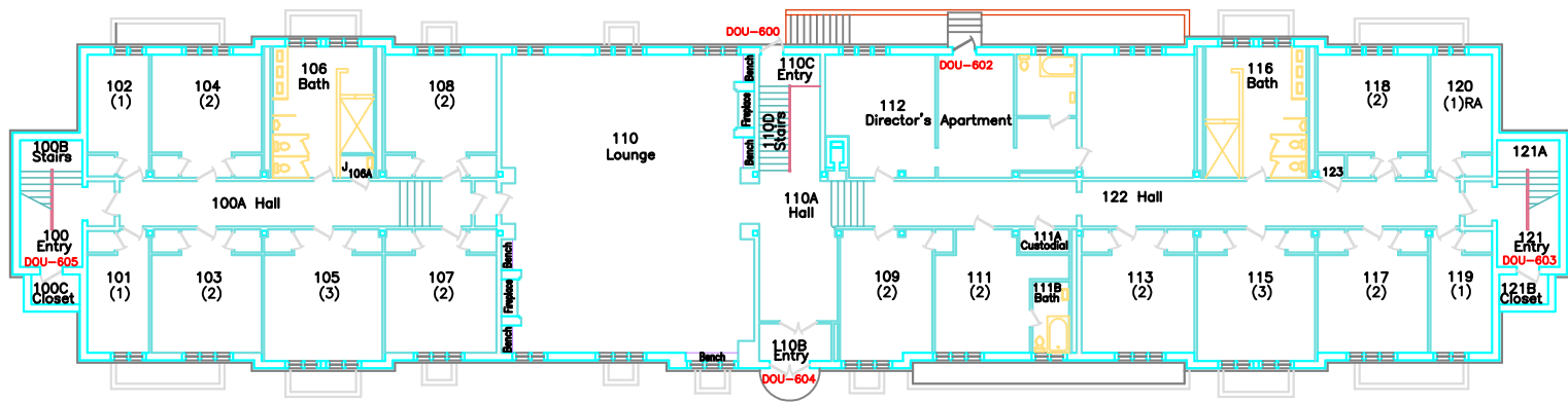
FIRST FLOOR
